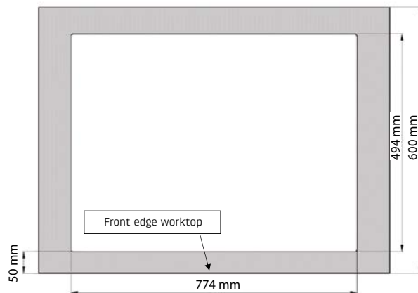
Flush-mounted installation without rebate
