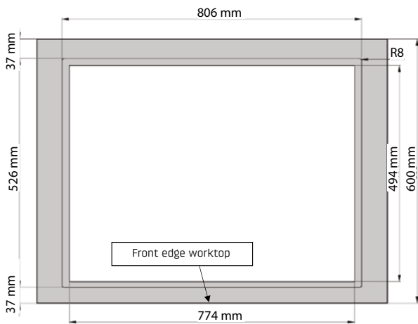
Flush-mounted installation with rebate
