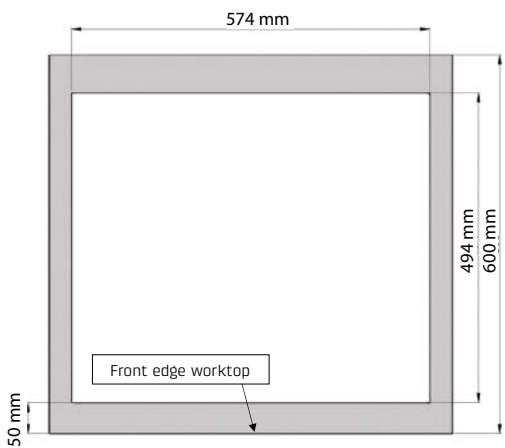
Flush-mounted installation without rebate
